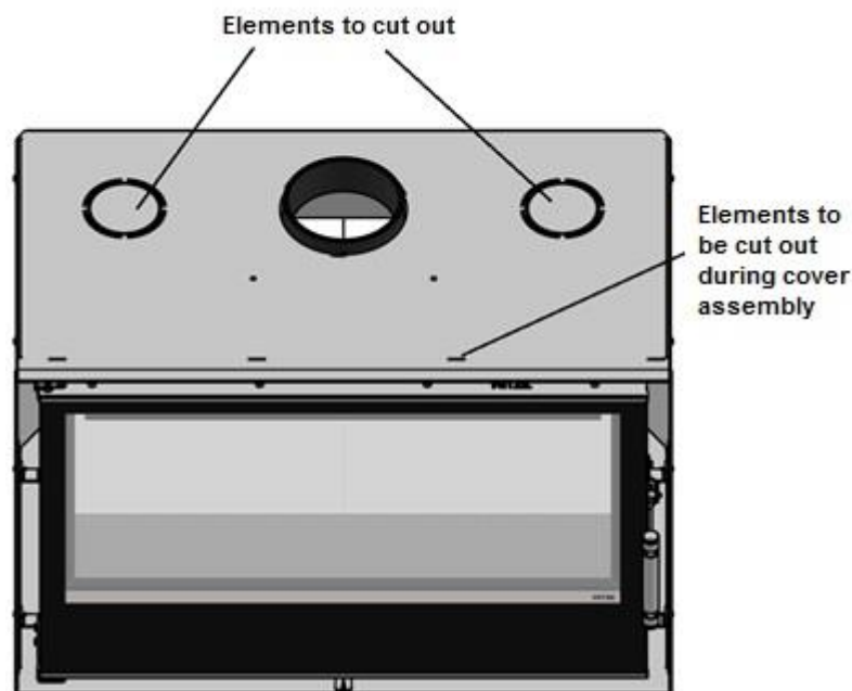
Fig. 8. Places of cutting before mounting connector when connecting the hot air distribution system.
