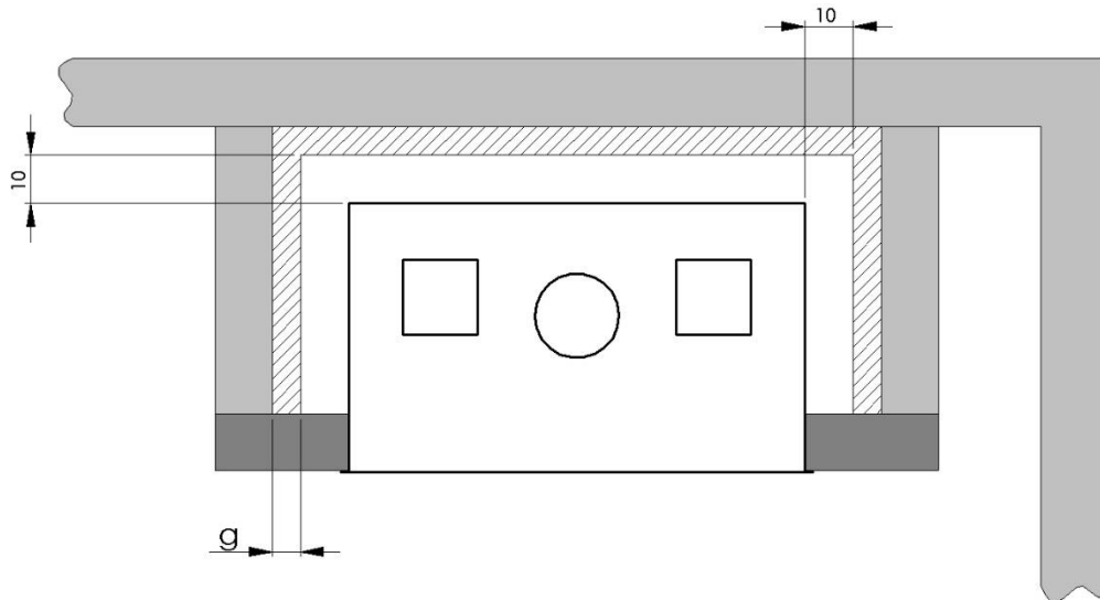
Fig. 5. Cassette housing - inflammable walls and insulation
