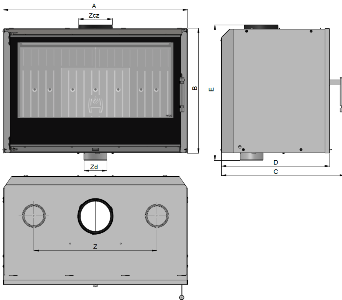
Fig. 2. Basic dimensions of CUBO fireplace cassettes
